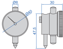
dial indicator
